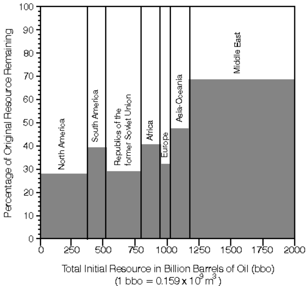
Figure 15B: Distribution of Earth's petroleum resources remaining by 2010, assuming no increase in current rates of utilization. Source: Masters, C. D.; Root, D. H.; and Attanasi, E. D. 1991. "Resource Constraints in Petroleum Production Potential." Science . vol. 253. 12 July 1991. pp. 146-152.
