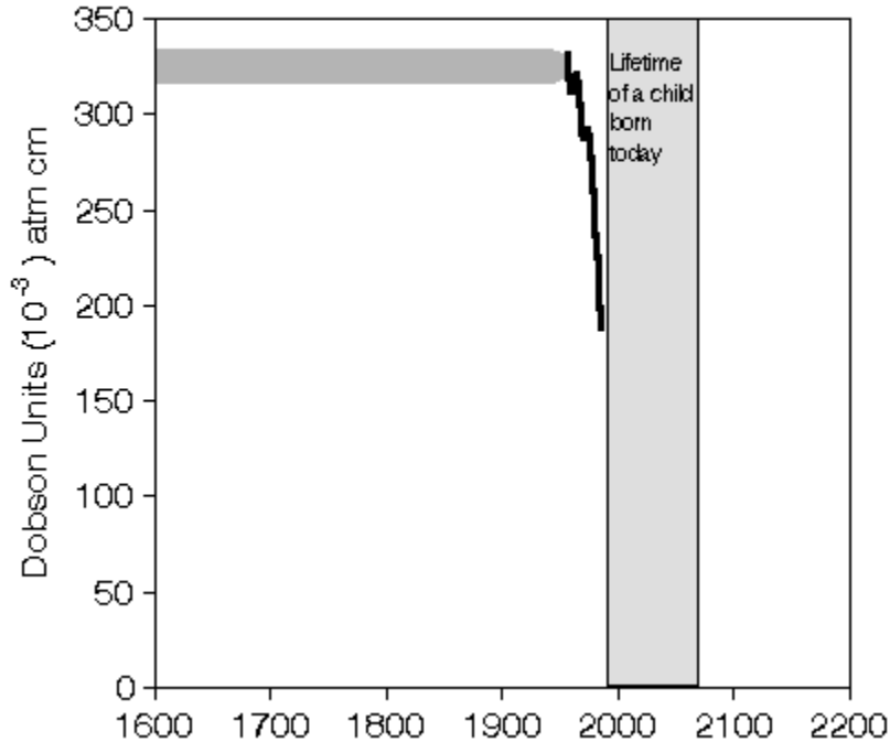
Figure 20: Total ozone concentrations above Halley Bay, Antarctica.
