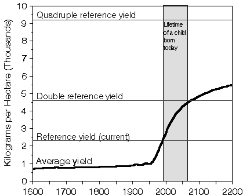
Figure 12: World agricultural yields from 1600 to present and projections. Sources: For the history: Food and Agriculture Organization, Production Yearbooks ; and U.S. Department of Agriculture, Agricultural Statistics . For the projection: Ruttan, V. W. 1990. "Constraints on Sustainable Growth in Agricultural Production: Into the 21st Century." In: Agriculture and Rural Development Department and Training Division, World Bank, eds. 1991. Eleventh Agricultural Symposium: Agricultural Issues in the Nineties . Washington: The World Bank; and Ruttan, V. W. December 1992. Personal communication.
