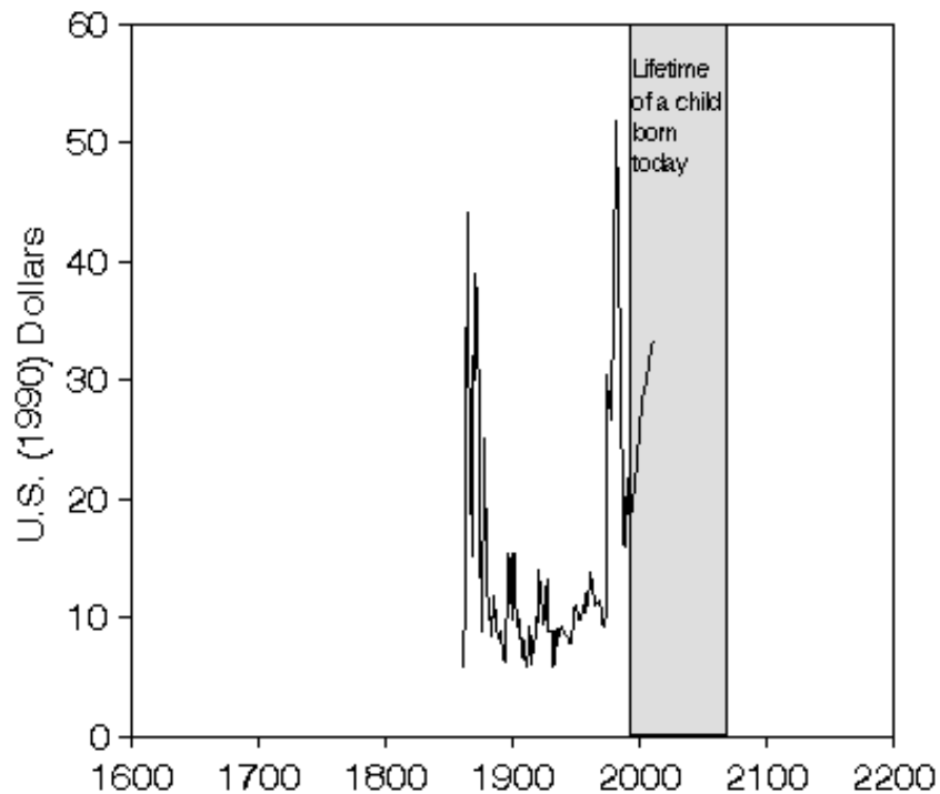
Figure 17: International price of imported crude oil from 1860 (first commercial oil production) to the present and a mid-level projection, 1990-2010. Source: Energy Information Administration. 1992. Annual Energy Outlook 1992 . Washington: U.S. Department of Energy. DOE/EIA-3083 (92). p. 6; and Oak Ridge National Laboratory. 1989. Energy and Technology R&D--What Could Make a Difference? as reported in: U.S. Department of Energy. 1991. National Energy Strategy . Washington: U.S. Government Printing Office.
