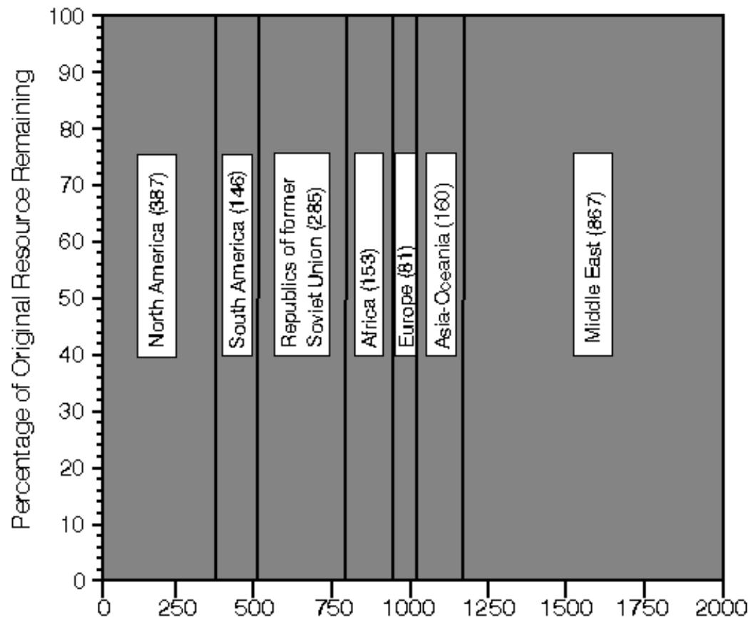
Figure 15A: Distribution of Earth's original (1900) total petroleum resource.
