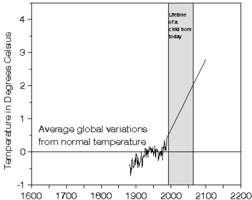
Figure 19: Average global variations from normal temperature, 1880-1988 and projection to 2100. Projections are from Scenario IS92a as presented in Intergovernmental Panel on Climate Change. 1992. 1992 IPCC Supplement . Nairobi: U.N. Environment Programme. p. 25. The historical data are from Hanson, J. E. 1988. As reported in Shabecoff, P. "Global Warming Has Begun, Expert Tells Senate." The New York Times . 24 June 1988. p. A1.
