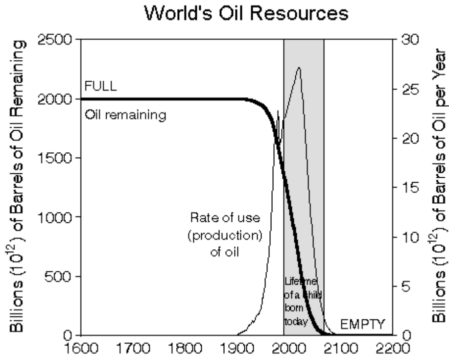
Figure 16: Exhaustion Cycle of the World's Oil Resources. Sources: Masters, C. D.; Root, D. H.; and Attanasi, E. D. 1991. Resource Constraints in Petroleum Production Potential. Science . vol. 253. 12 July 1991. pp. 146-152. DeGolyer and MacNaughton. 1992. Twentieth Century Petroleum Statistics . Dallas: DeGolyer and MacNaughton. p. 4.
