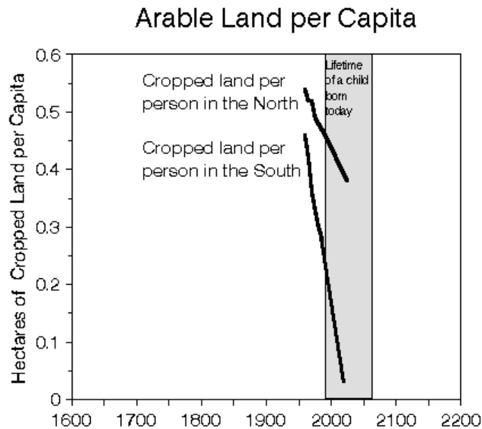
Figure 10: Cropped arable land per capita, actual and projected. The projections are linear extrapolations. Source of historical data: U.N. Food and Agriculture Organization. 1989. FAO Production Yearbook tapes. Rome: U.N. Food and Agriculture Organization.
